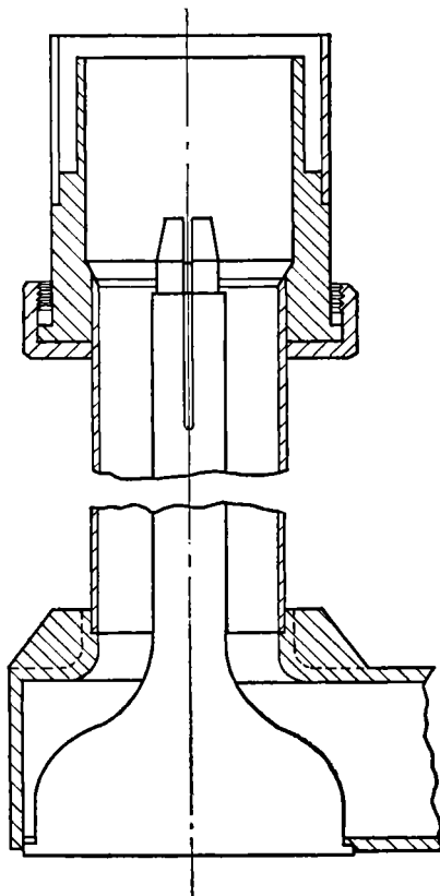
FIG. 11-16.—10-cm, 800-kw pulse-power “doorknob” transition for 1\frac{1}{8} -in. coaxial line to 1\frac{1}{2} - by 3-in. waveguide.
